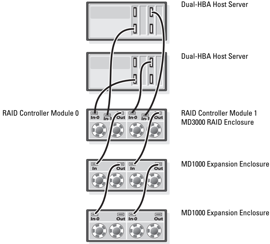
Figure 1-5. Cabling in a Direct-attached SAS Cluster
